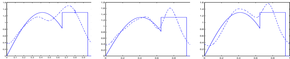
FIGURE 2. Examples of estimators \widehat{f}_n^{STCV} obtained on 2^{10} observations. The true distribution is represented in dashed lines. Figures from left to right correspond respectively to Case 1 , Case 2 and Case 3 .
