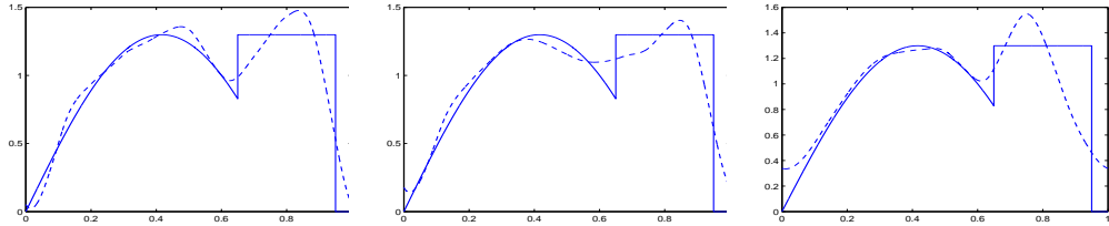
FIGURE 1. Examples of estimators \widehat{f}_n^{HTCV} obtained on 2^{10} observations. The true distribution is represented in dashed lines. Figures from left to right correspond respectively to Case 1 , Case 2 and Case 3 .
